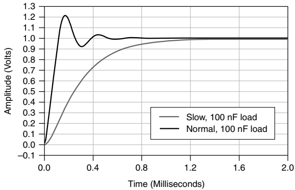
Figure 4. 1 mA Range, 100 nF Load Step Response, Nominal
